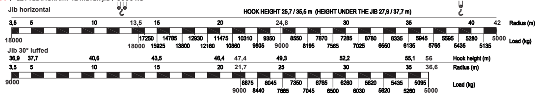
2 HEAVYLIFT / LØFTEDIAGRAM: 42 METER JIB / 5000 KG
